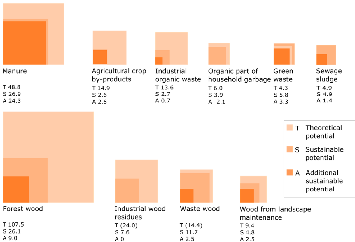
Figure 3: Primary energy potential of all 10 biomass types in petajoules PJ per year.
