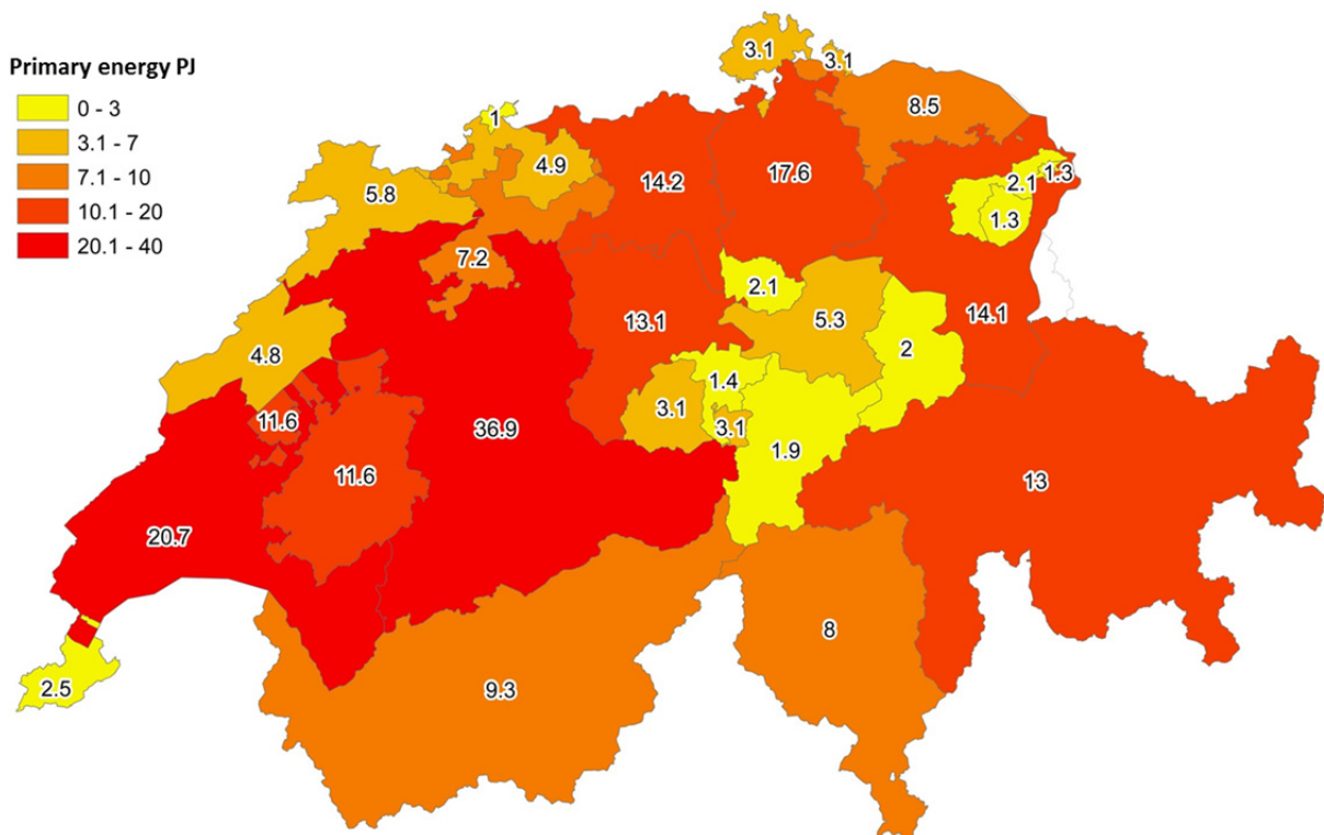
Figure 4: Spatial distribution of the theoretical primary energy potentials in petajoules PJ per year of all 10 biomass types according to canton.
