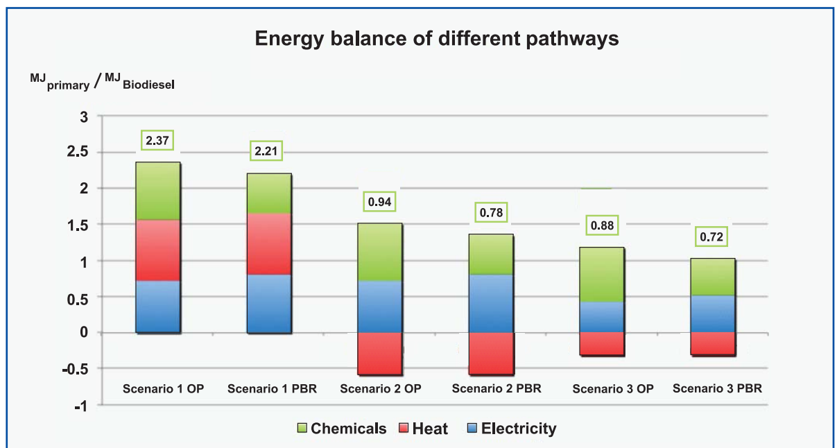
Figure 3. Preliminary results of energy balance. Courtesy Pierpaolo Cazzola, IEA Secretariat, Paris.
